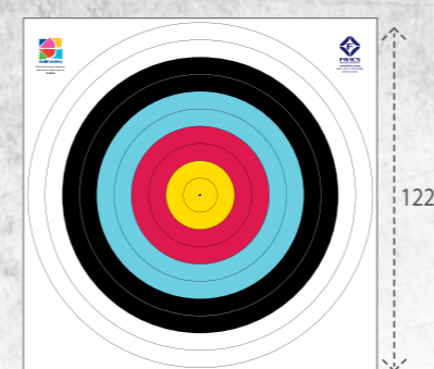
PT 001 OUTDOOR 122cm Target Face Range: 90m / 70m / 60m Mark dimension: 122cm X 122cm Total dimension: 125cm X 125cm (width/length)
